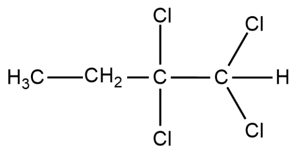
1,1,2,2-tetrachlorobutan
